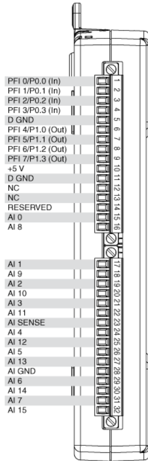
USB-6210 Pinout
