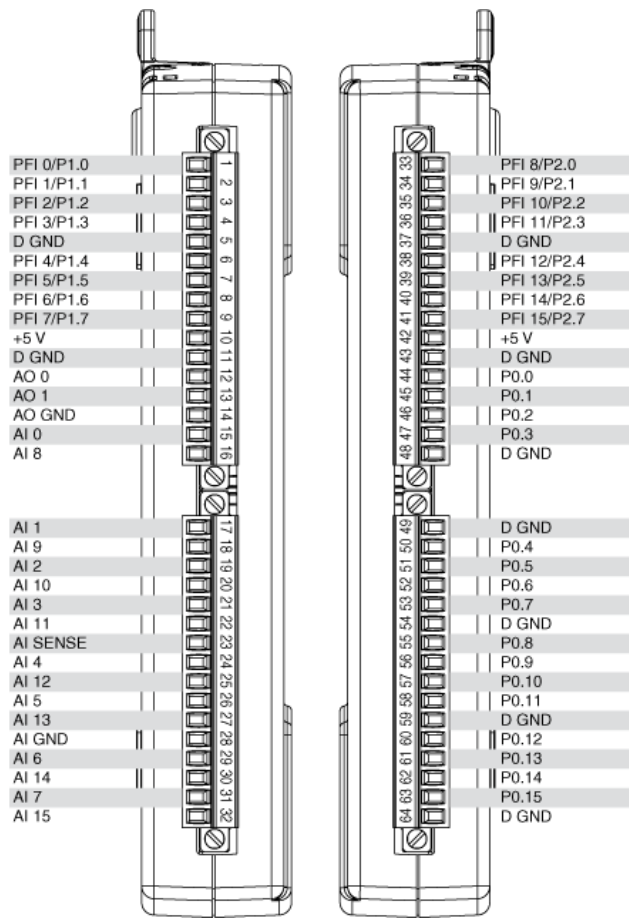
USB-6212/6216 Pinout
