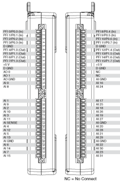
USB-6218 Pinout
